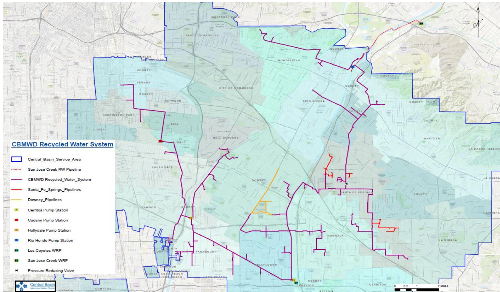
FIGURE 1 CBMWD EXISTING RECYCLED WATER FACILITIES (Fiscal Year 2020/2021) Central Basin Municipal Water District Recycled Water System
